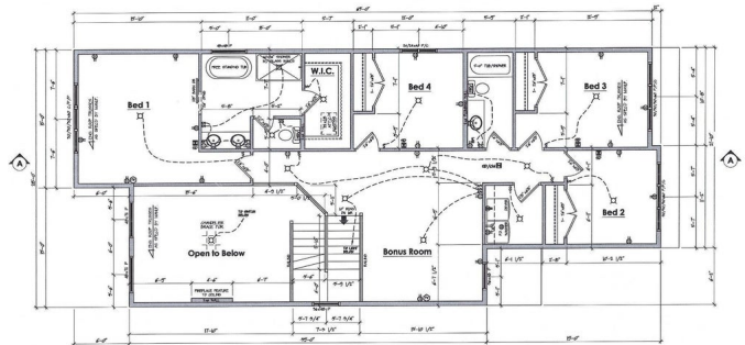
Second Floor Plan 1206 of 87' Ceiling
